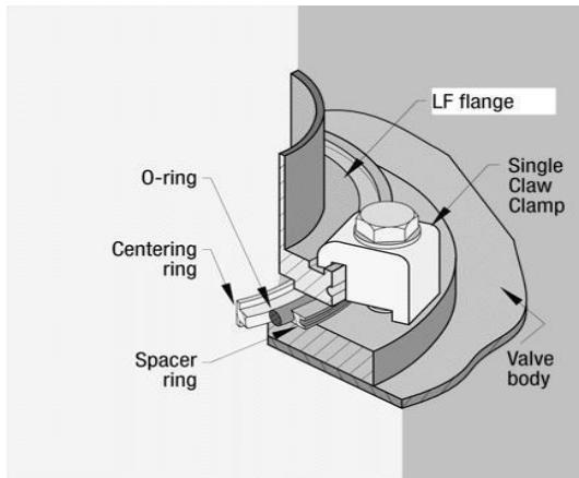
ISO-K assembly with single claw clamp
