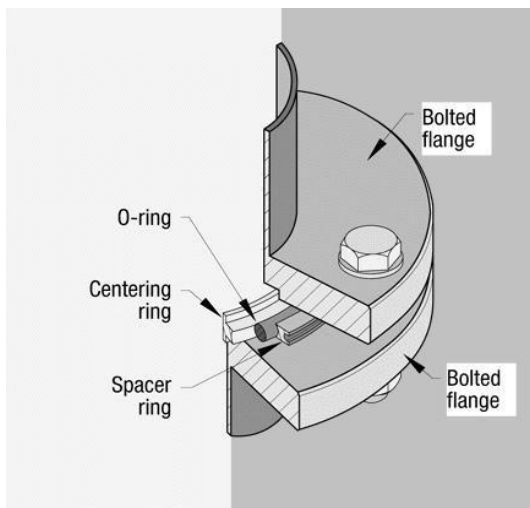
ISO-K assembly with bolted flanges
