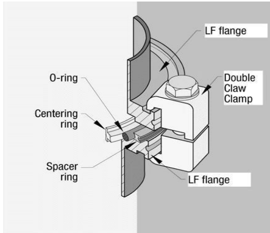
ISO-K assembly with double claw clamps
